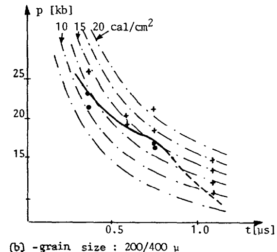
Fig 28 Sensitivity of granular RDX + detonation • no detonation
